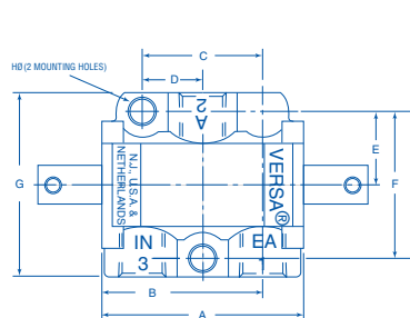
1/4" - 1/2" Body
