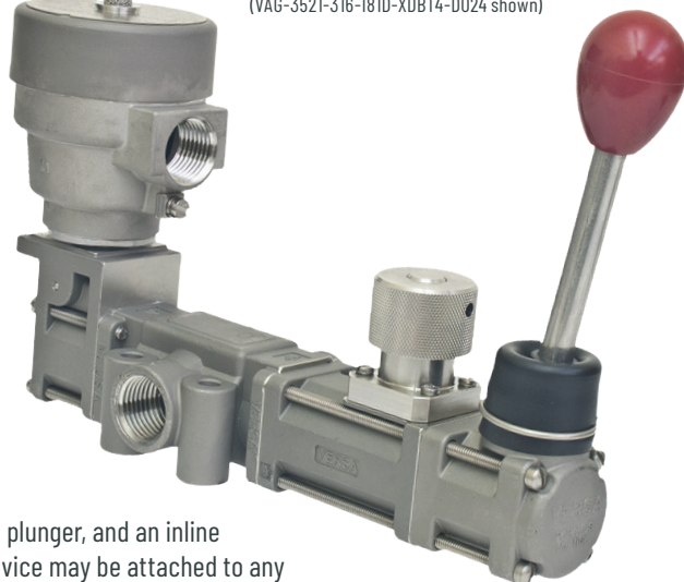
Latching/Manual Reset Three-Way Valve, Solenoid Actuated. (VAG-3521-316-181D-XDBT4-D024 shown)
