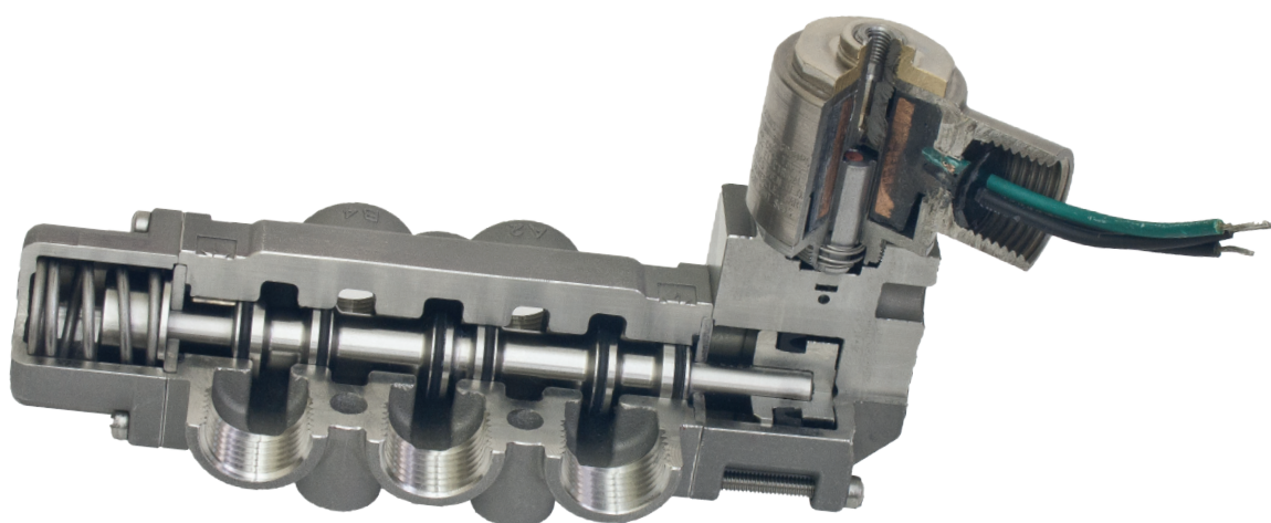
Shown: VSG-4522-316-PC-XX-D024
