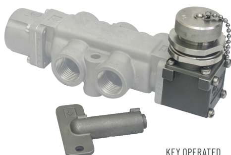
KEY OPERATED
