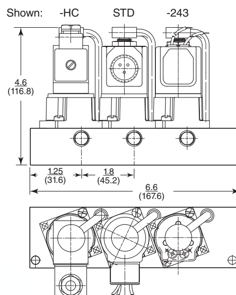
DIMENSIONS SHOWN IN INCH (MM)
