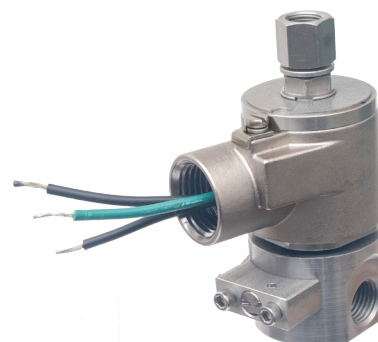
XT solenoid shown with: -H2E Hyd Adapter And -G5R Override
