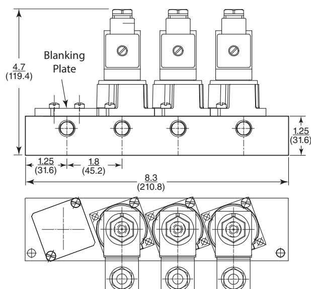
DIMENSIONS SHOWN IN INCH (MM)
