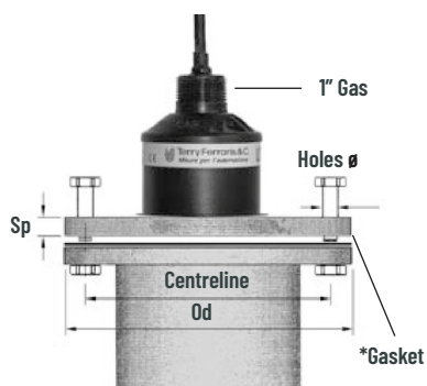
UTF in flanged execution
