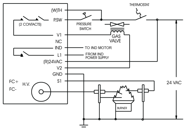
Figure 2. Remote Sense
