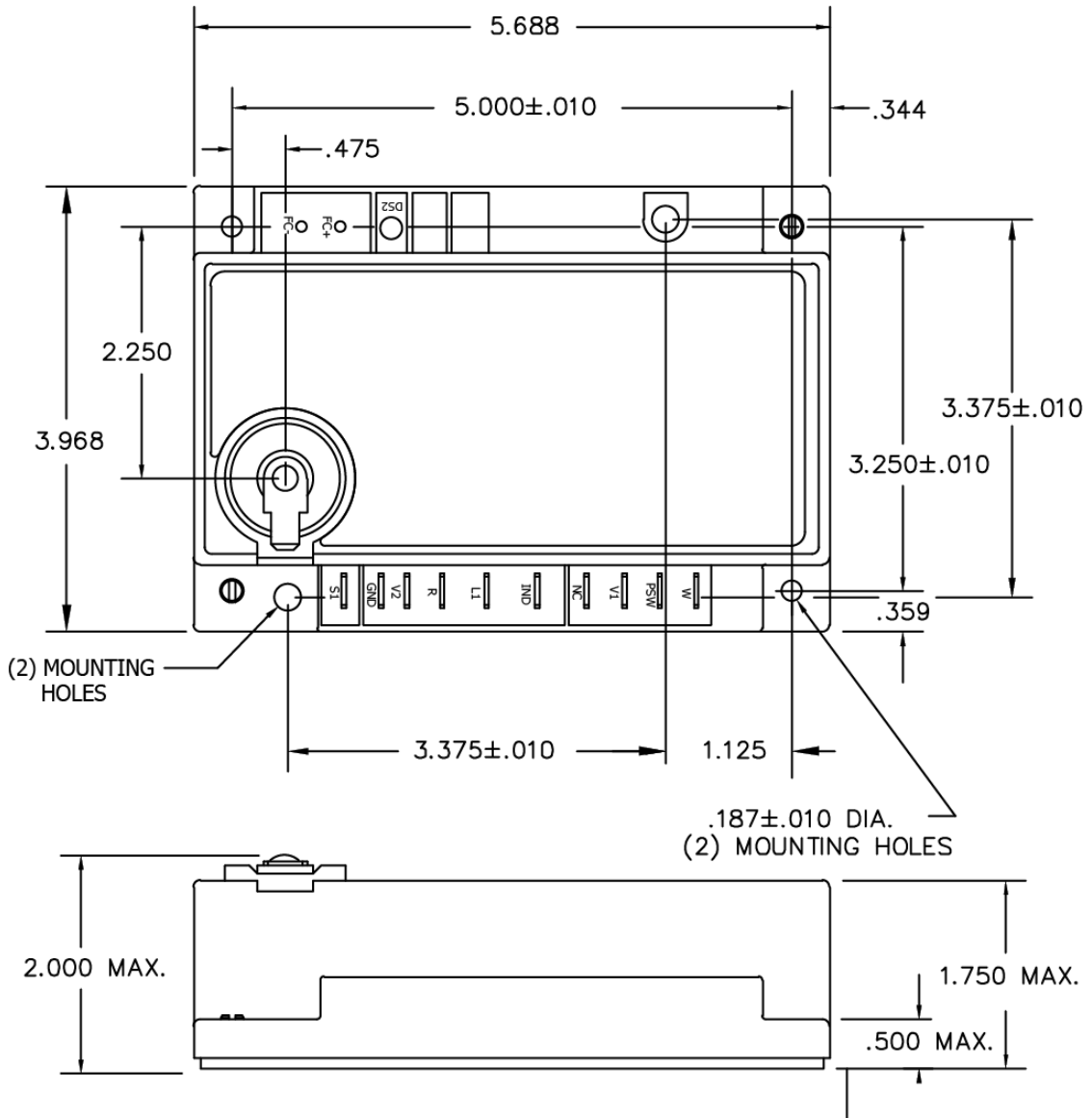
Figure 3. Standard Enclosure
