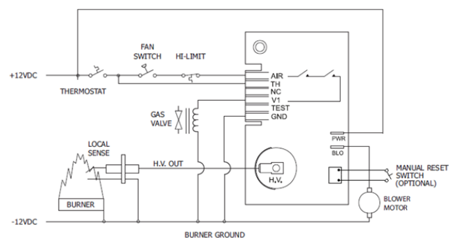
Figure 1. Local Sense with Blower Relay
