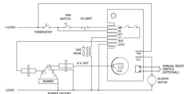
Figure 3. Remote Sense with Blower Relay
